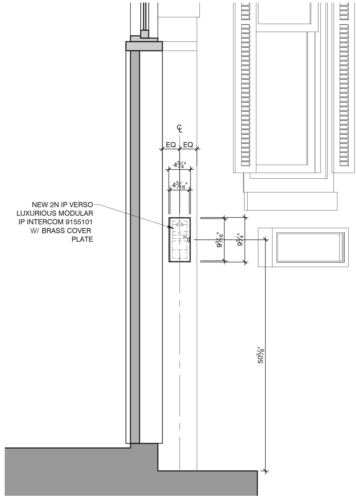
1 PROPOSED FRONT DOOR SIDE ELEVATION SCALE: 1" = 1'-0"
