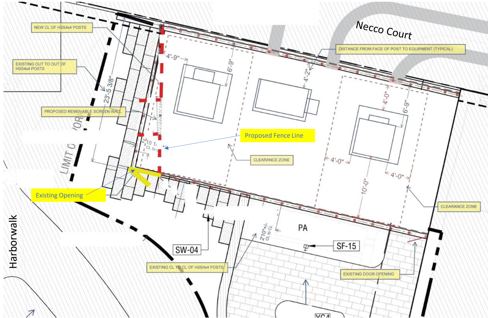
5 NECCO ST TRANSFORMER ENCLOSURE EXISTING CONDITIONS
