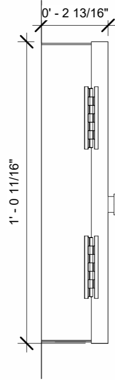
7 Left View 3" = 1'-0"
