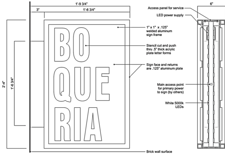
ELEVATION OF BLADE SIGN
