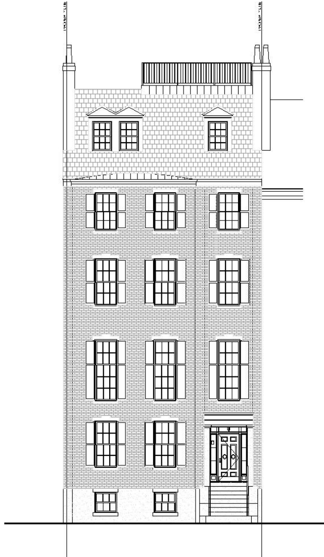
Proposed Front Elevation (previously presented to the BHAC)
