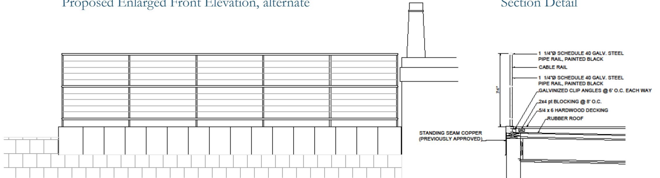
Proposed Enlarged Front Elevation
