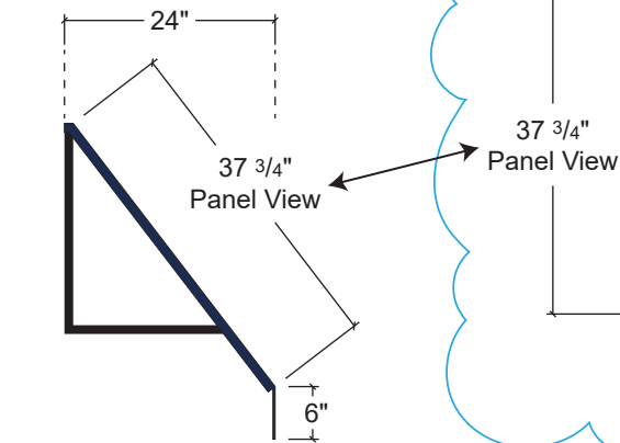
S1 Side View: Scale: 1/2" = 1'
