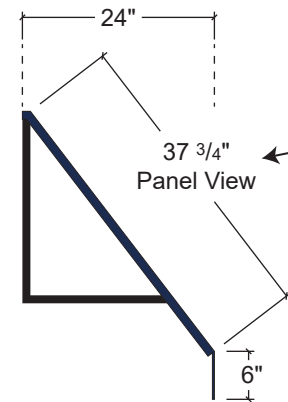
S2 Side View: Scale: 1/2" = 1'
