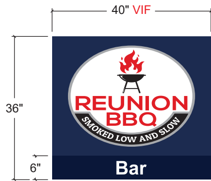
E2 Elevation: (Qty 1) Shed Awning Scale: 1/2" = 1'
