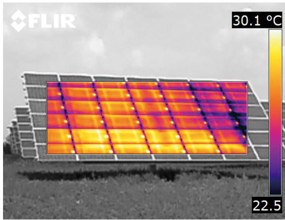
Hot solar panels Source: FLIR Media
