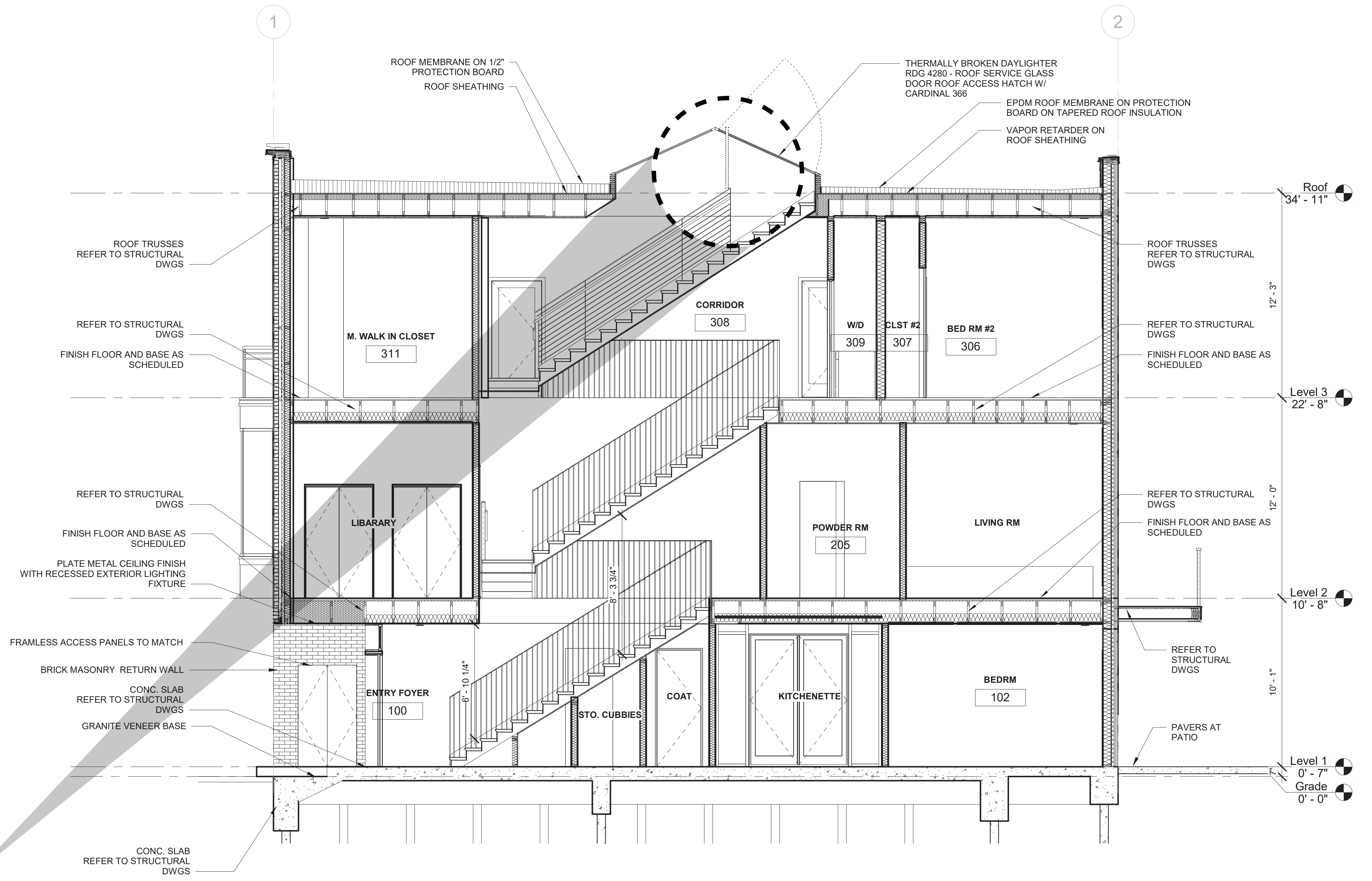
1 BUILDING SECTION - STAIR 1/4" = 1'-0"
