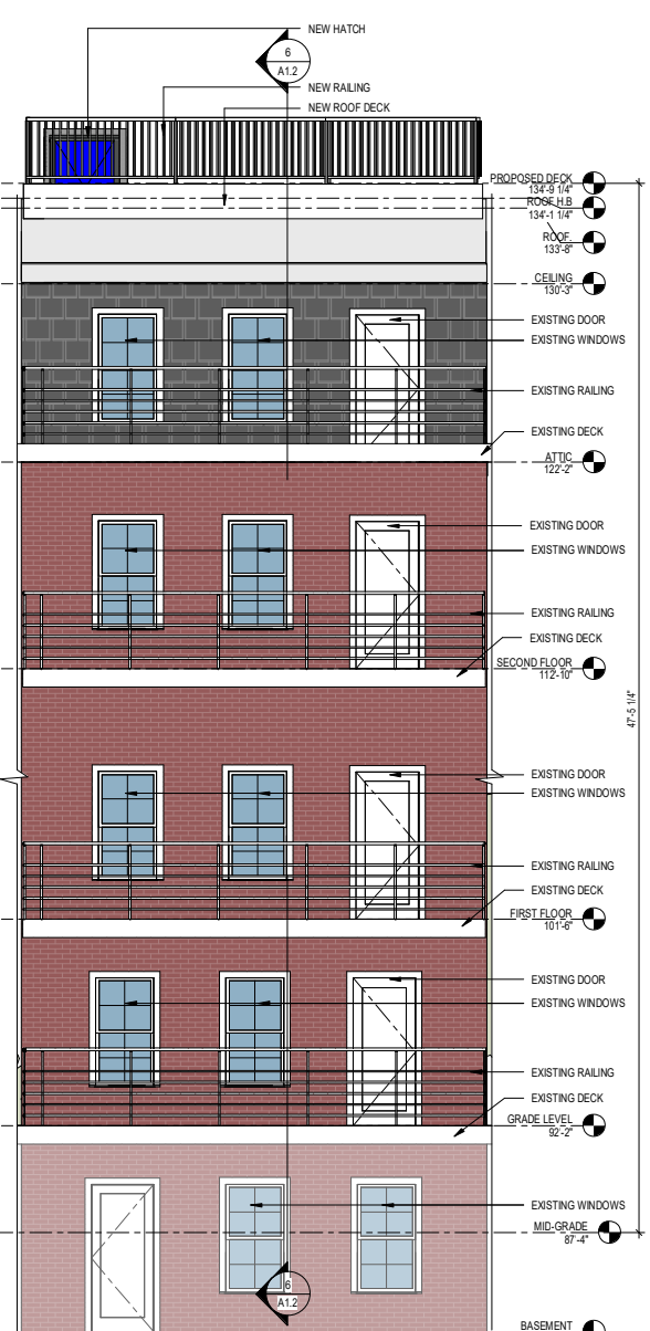
2 SOUTH ELEVATION PROPOSED 1/4" = 1'-0"
