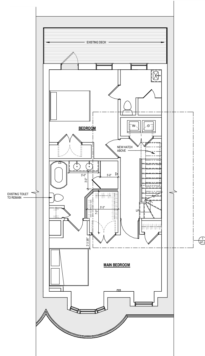
4 THIRD FLOOR PROPOSED 1/4" = 1'-0"
