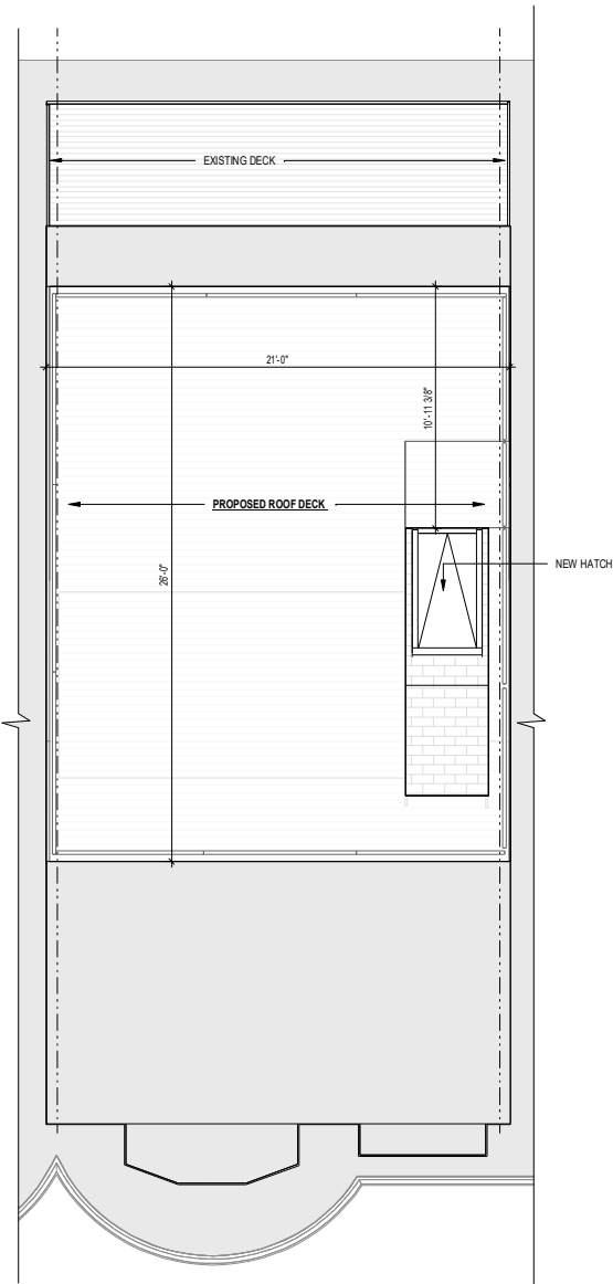
1 ROOF PLAN PROPOSED 1/4" = 1'-0"
