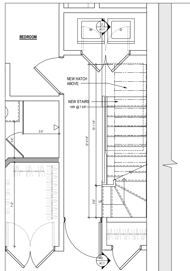
1 PARTIAL THIRD FLOOR PROPOSED 1/2" = 1'-0"
