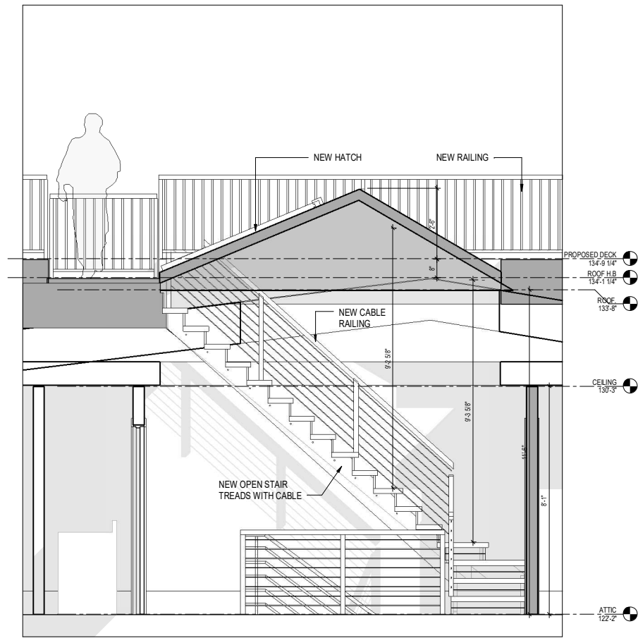
2 STAIR SECTION 1/2" = 1'-0"
