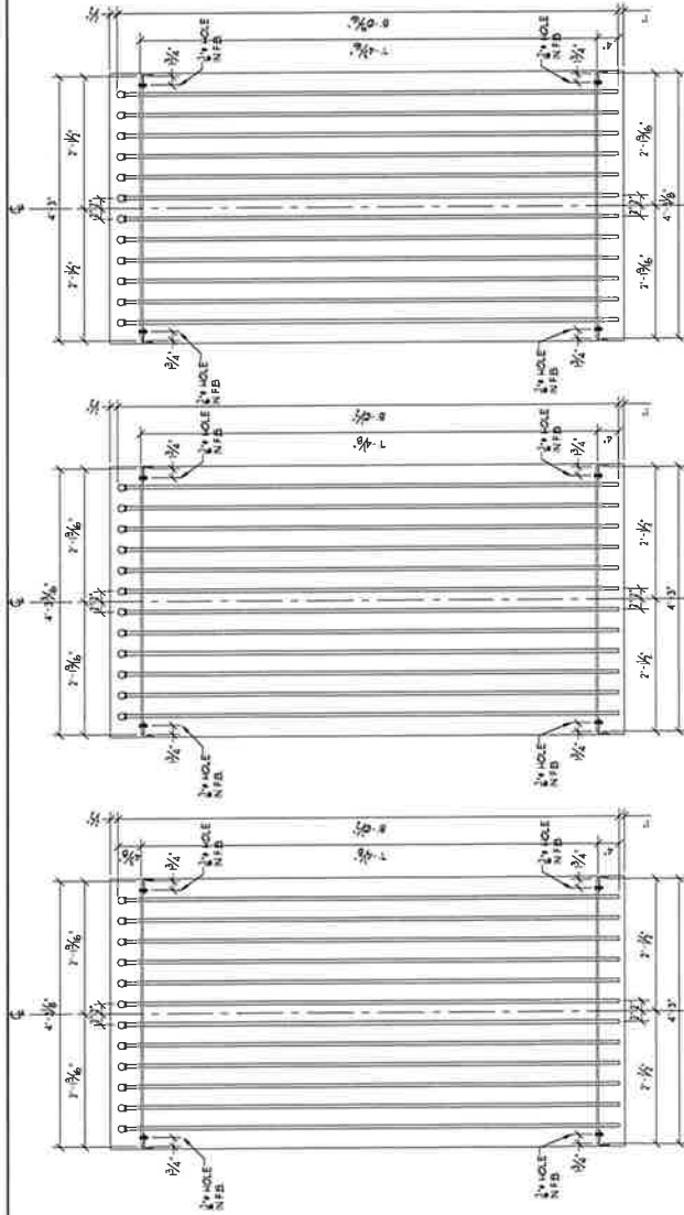
GR1 MAKE - (1) SCALE 1" = 1'-0"
