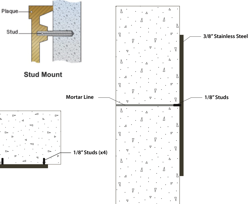
A.4 TOP-DOWN VIEW DETAIL Scale: 1:2
