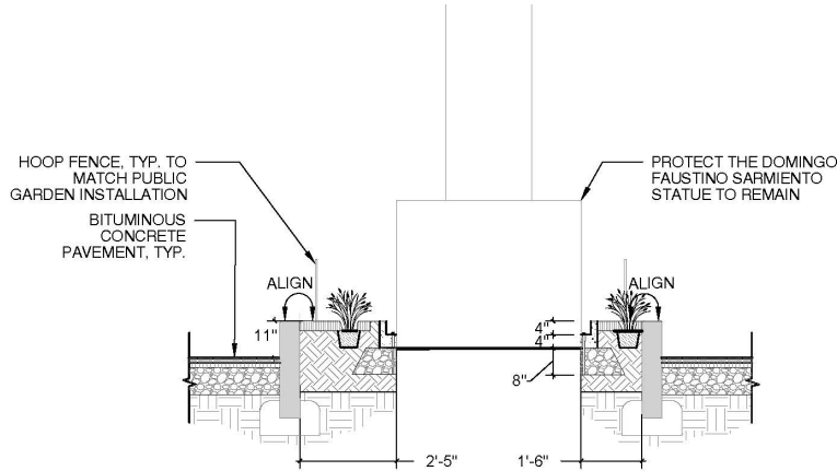
A SARMIENTO STATUE- NORTH / SOUTH SECTION WITH EXISTING CURB PLACEMENT SCALE: 1" = 3'-0"
