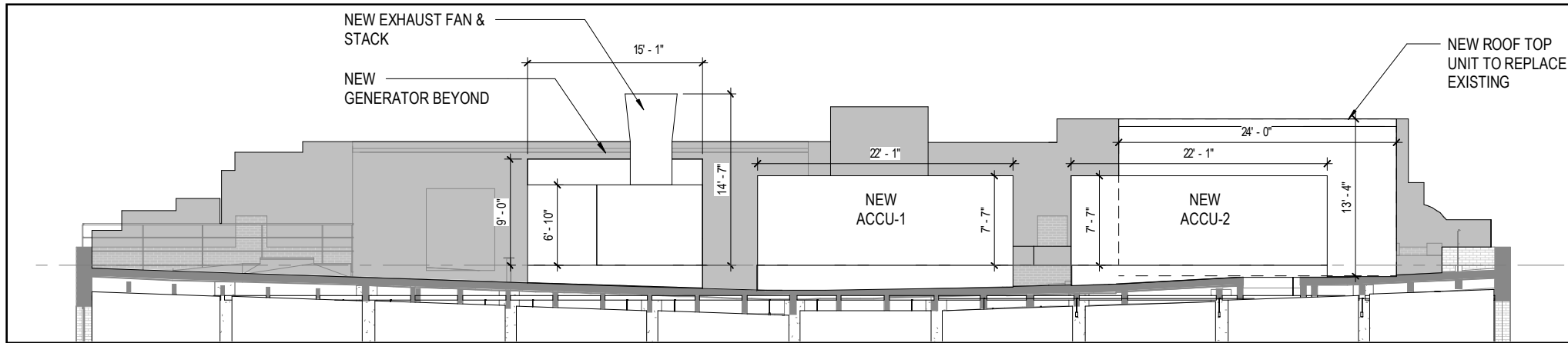
ROOFTOP SECTION 2 - PROPOSED
