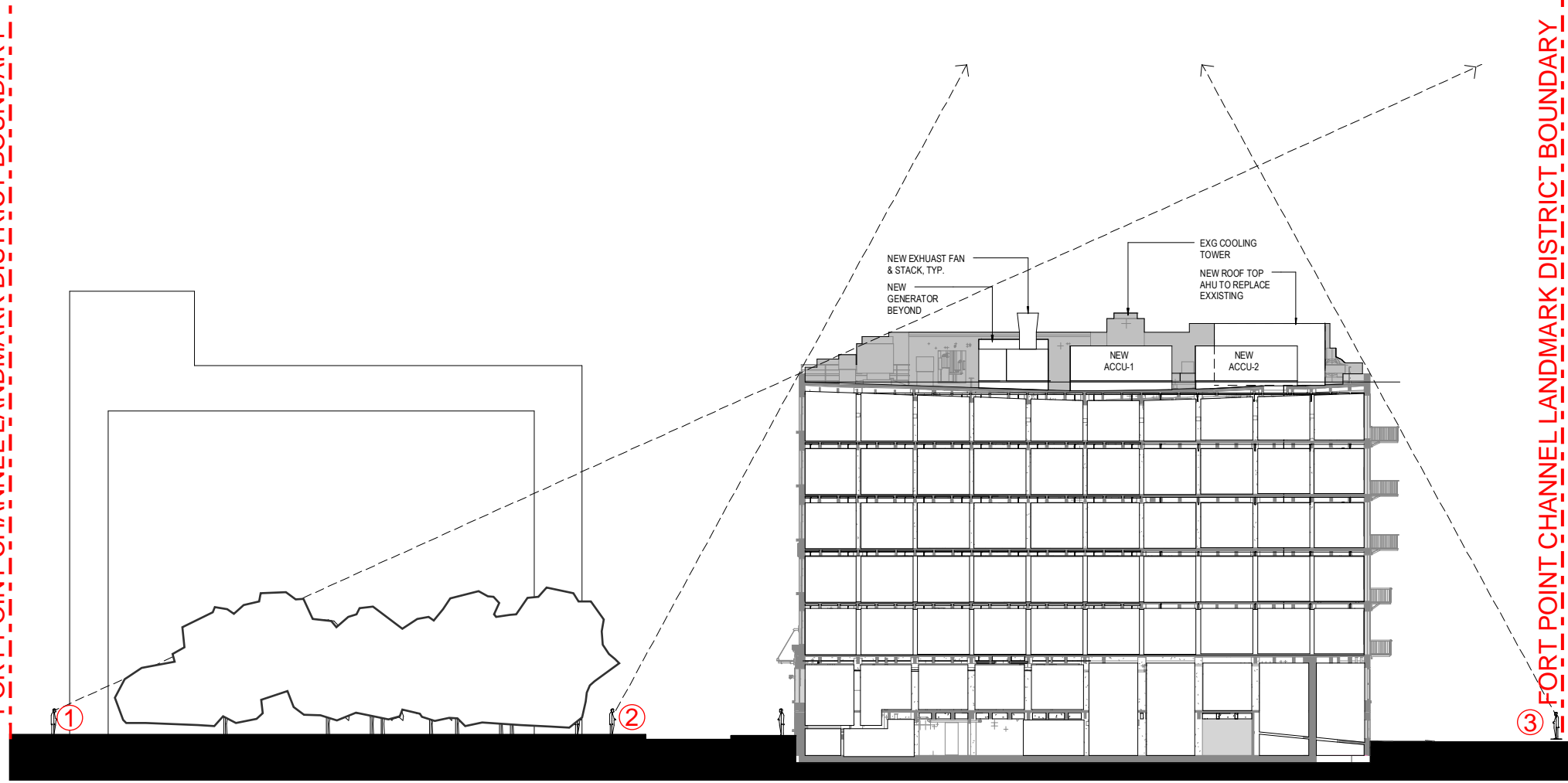
SITE SECTION 1 - WITH SIGHT LINES
