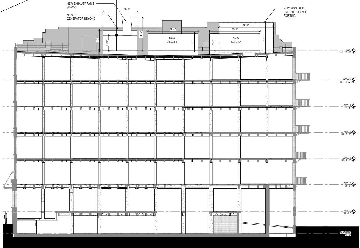
BUILDING SECTION 2 - EXISTING
