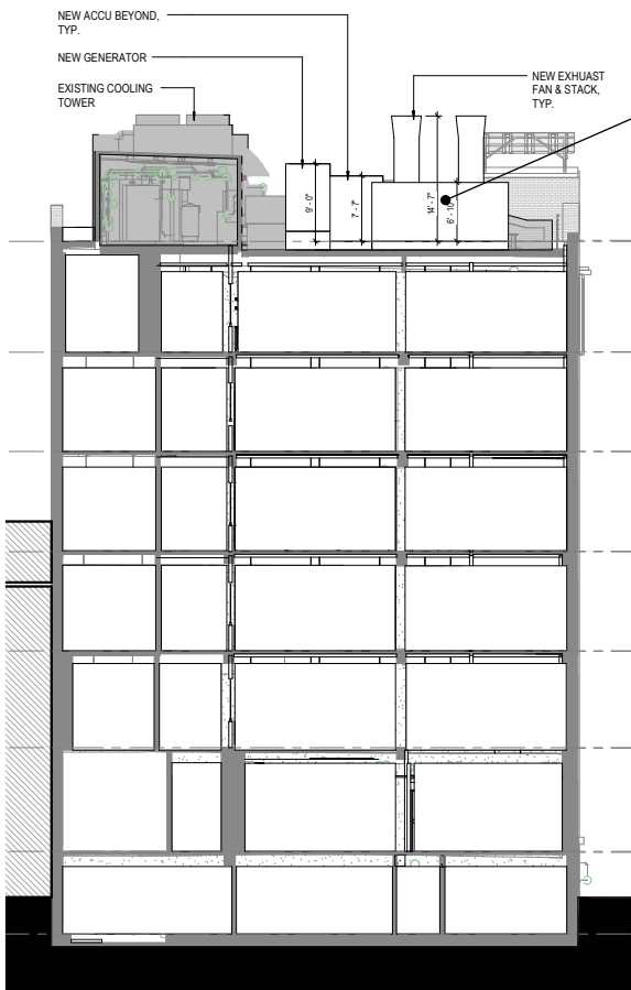
BUILDING SECTION 1 - PROPOSED
