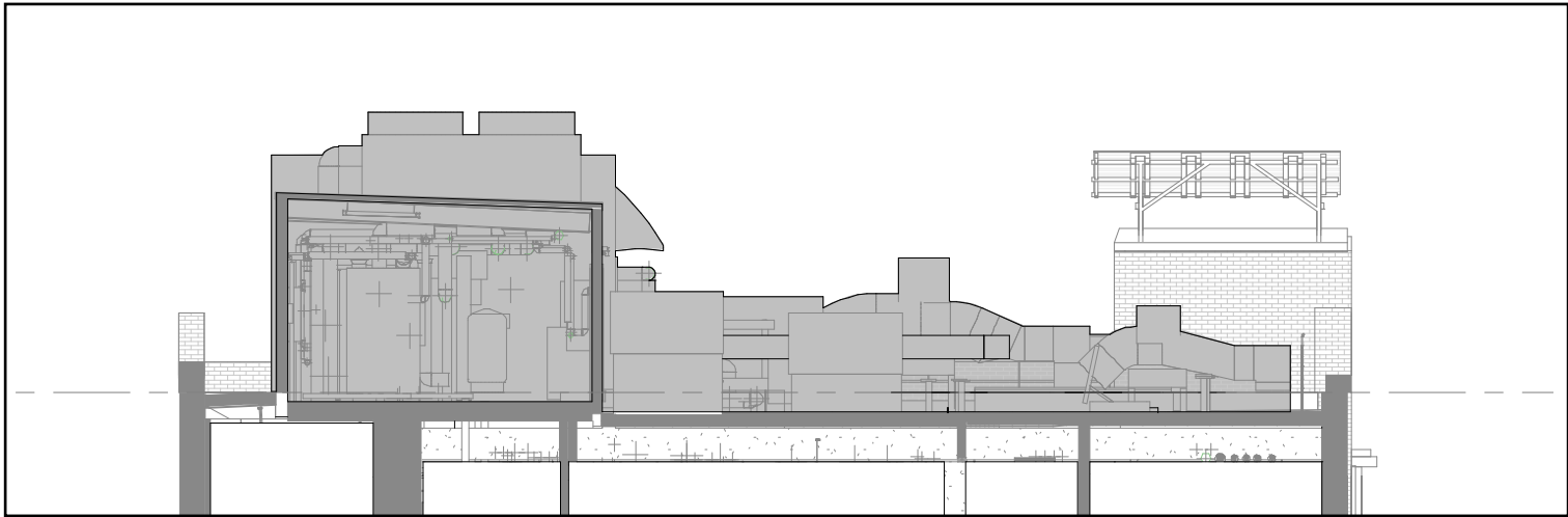
ROOFTOP SECTION 1 - EXISTING
