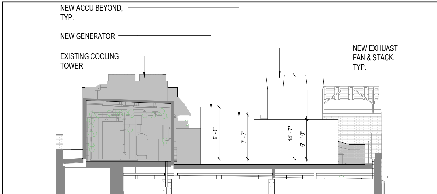
ROOFTOP SECTION 1 - PROPOSED
