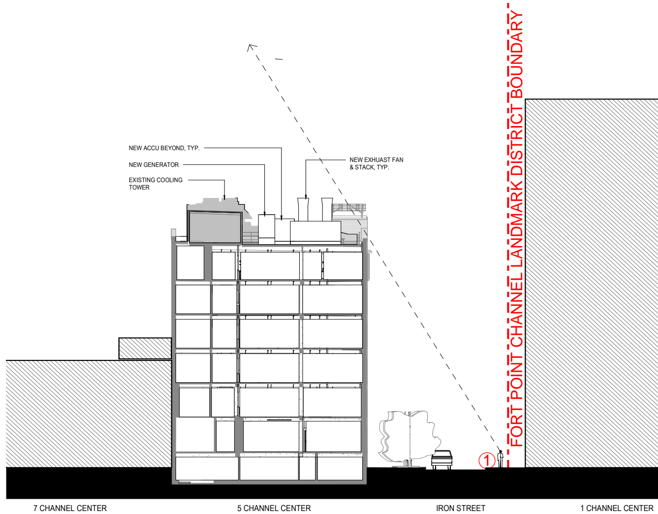
SITE SECTION 2 - WITH SIGHT LINES
