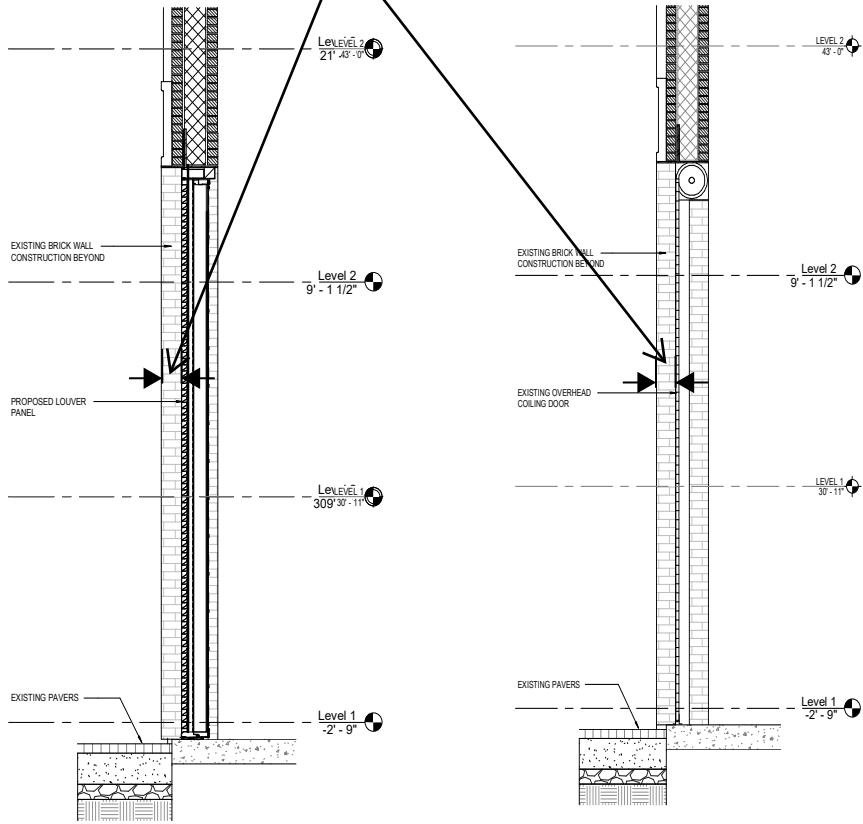
BUILDING SECTION 1 - DETAIL THROUGH PROPOSED EXISTING OVERHEAD DOOR
