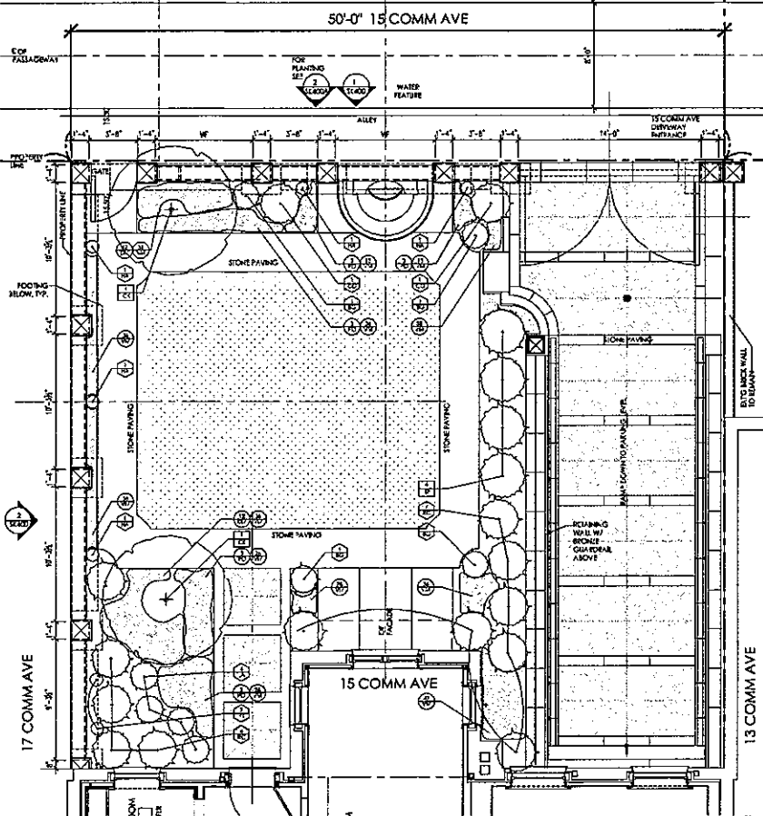
1 REAR YARD PLAN 1/4" = 1'-0"
