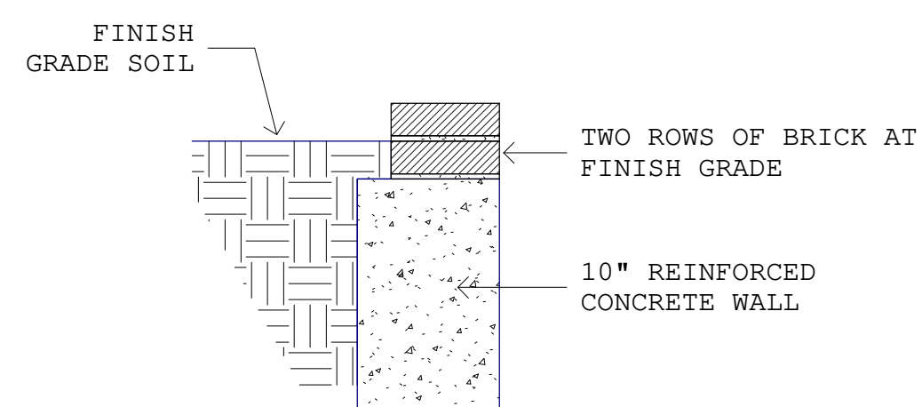
2 TOP OF WINDOW WELL 1" = 1'-0"
