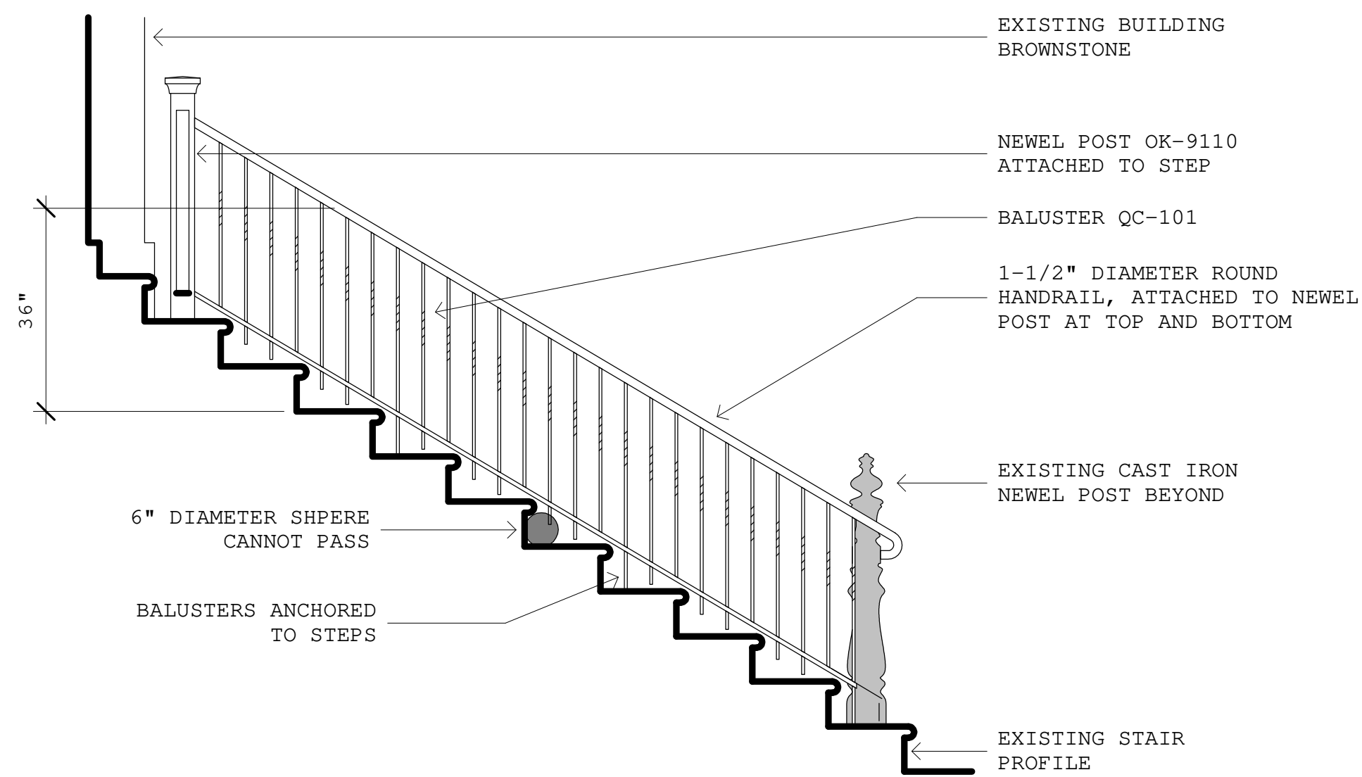
3 FRONT EXTERIOR STAIR RAILING 'B' 1/2" = 1'-0"
