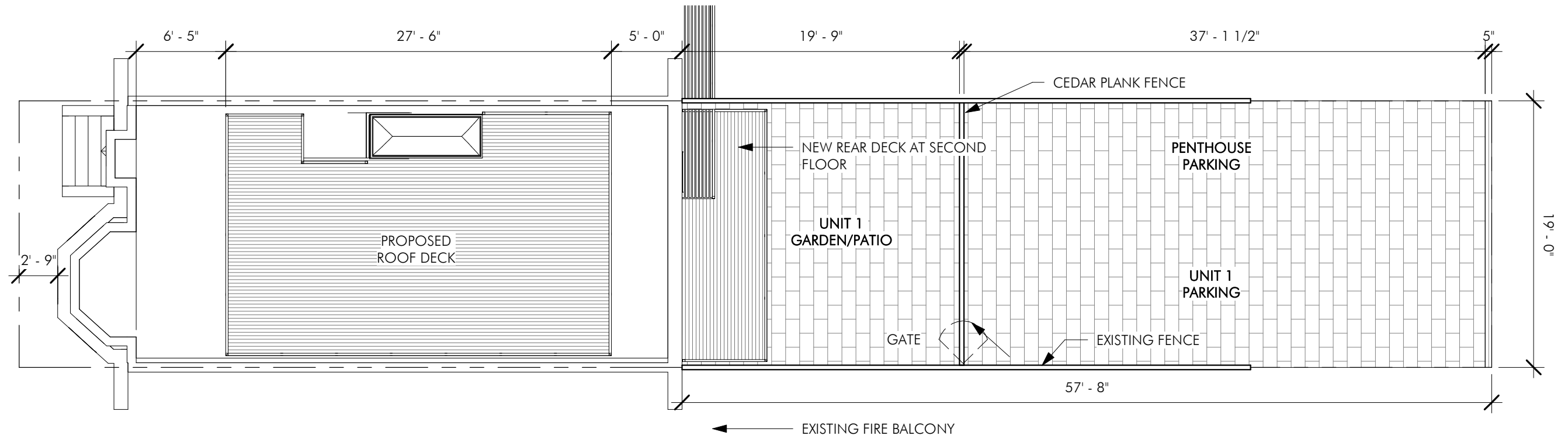
SITE PLAN
