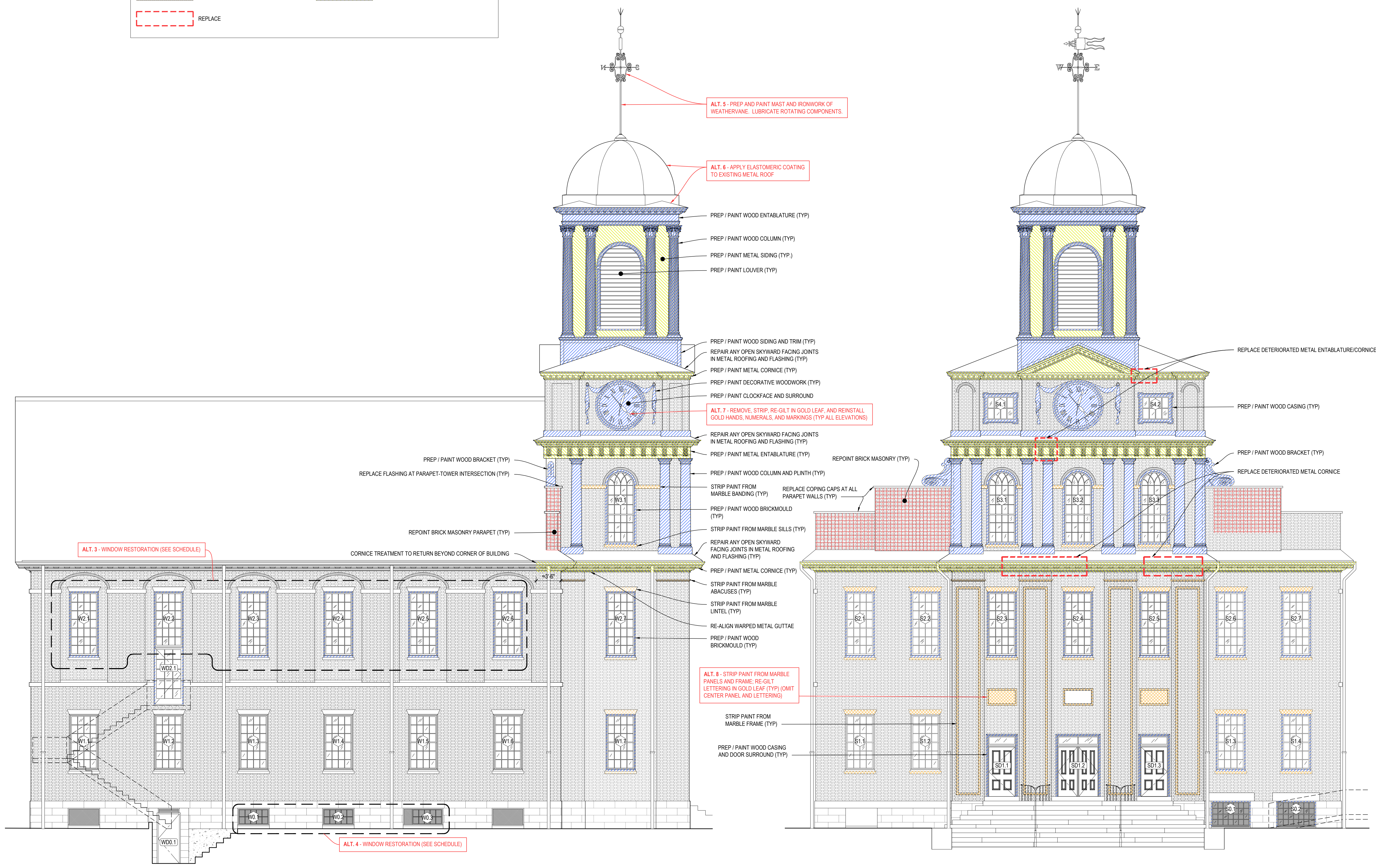
02 EXTERIOR ELEVATION: WEST NOT TO SCALE
