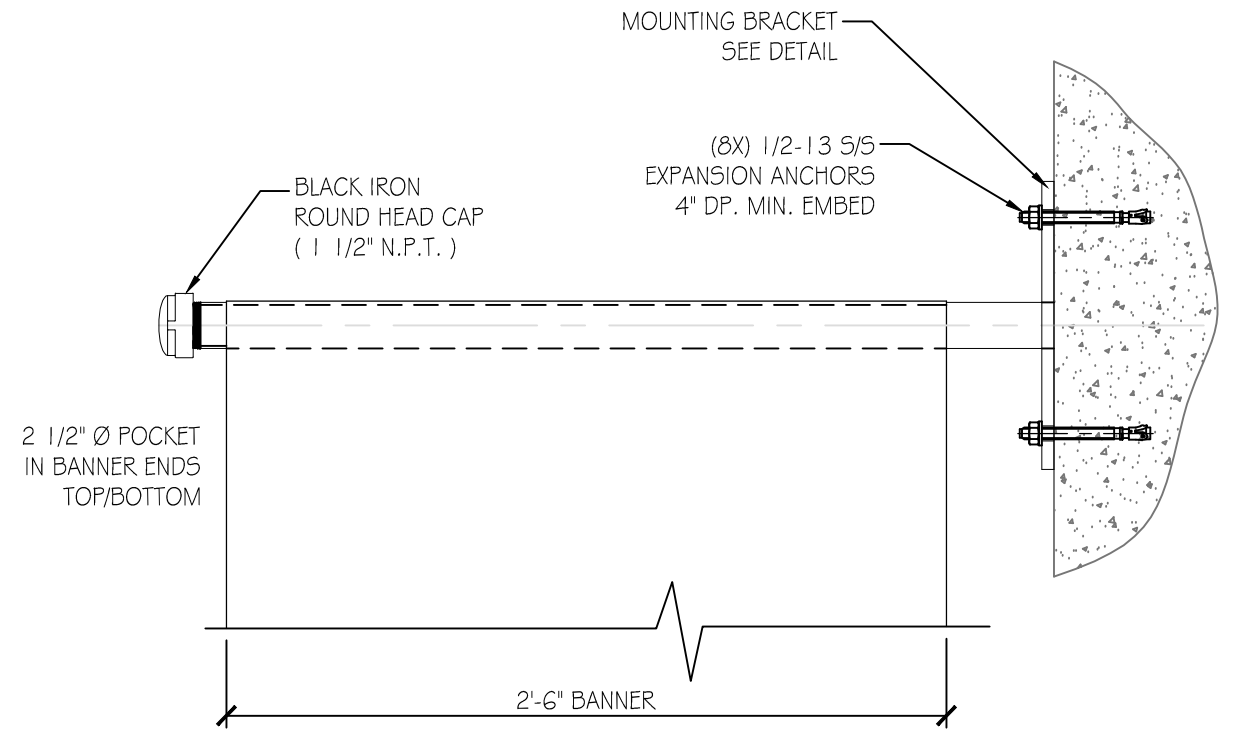
DETAIL VIEW SCALE: 1 1/2" = 1'-0"
