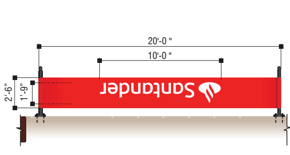
1 NEW D/F FLAG SIGN 50 sq. ft. SCALE: 3/16" = 1'-0" Qty 1
