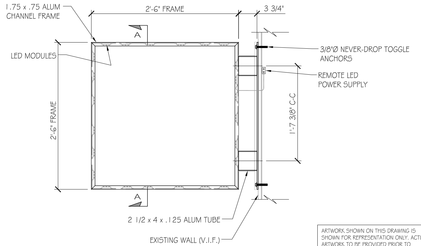
FRAMING DETAIL SCALE: 1" = 1'-0"
