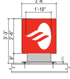
2 NEW D/F BLADE SIGN 6.25 sq. ft. SCALE: 3/16" = 1'-0" Qty 1
