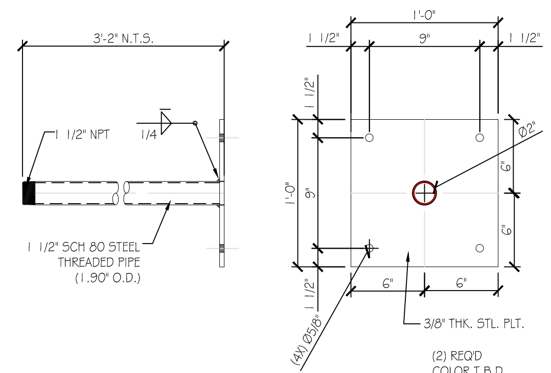
MOUNTING BRACKET DETAIL SCALE: 1 1/2" = 1'-0"
