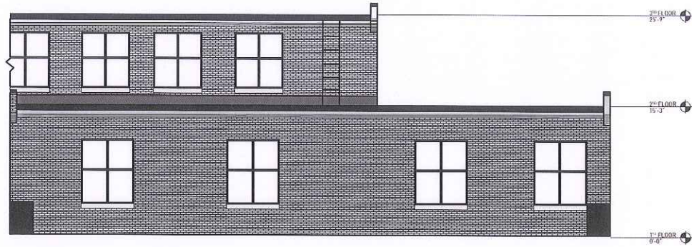
① EXTERIOR ELEVATION - EXISTING 3/32" = 1"
