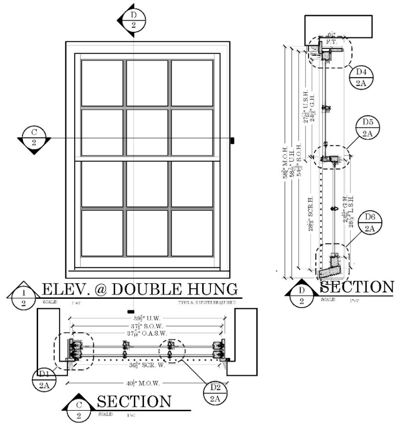
Proposed window replacement in kind
