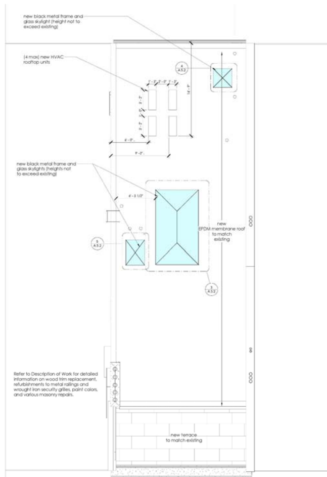
Proposed Roof Plan with Skylight Replacements
