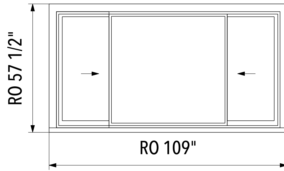
20 Proposed window elevation
