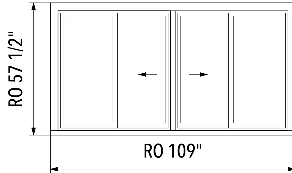
10 Existing window elevation
